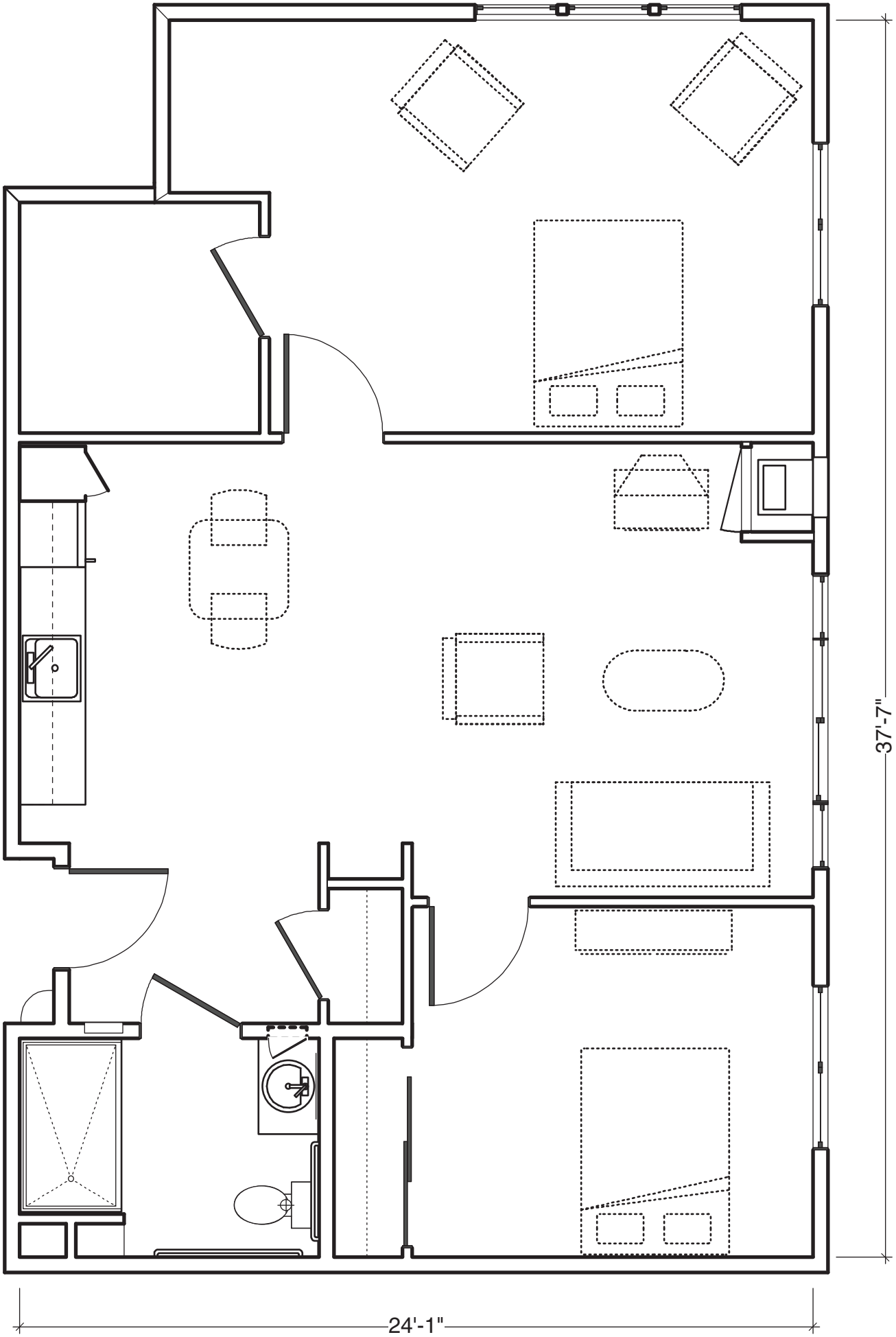
1 ASSISTED LIVING – 2 BEDROOM Scale: 1/4" = 1'-0"
